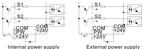
Figure 3-13 PNP modes
