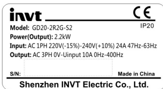
Figure 2-1 Name plate
