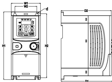
Wall mounting of 0.75~2.2kW inverters
