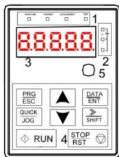
Figure 4-2 External keypad
