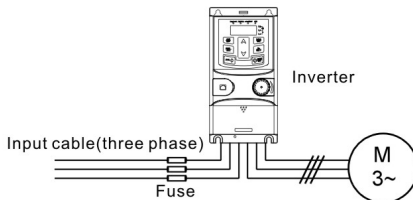
Figure 3-14 Fuse configuration
