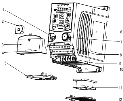
Figure 2-3 Product structure (Three phase 380V, \leq 2.2\text{kW} )
