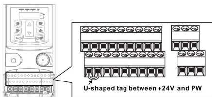
Figure 3-11 U-shaped contact tag
