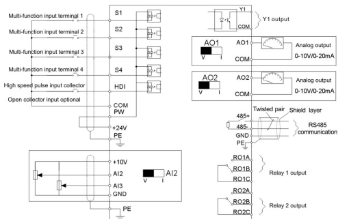
Figure 3-9 Wiring of control circuit
