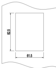
Installation dimension
